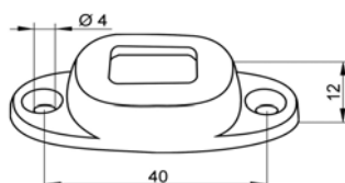
5123-011-4
