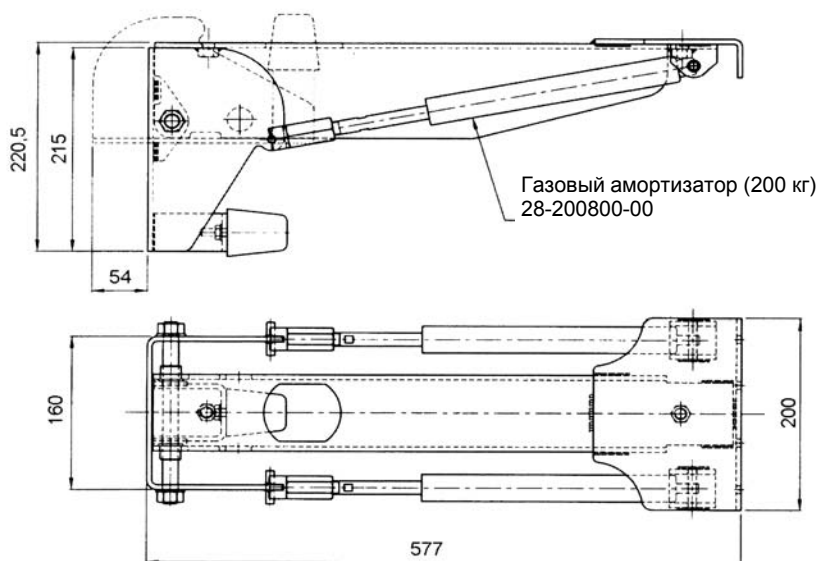
5124-010-0
